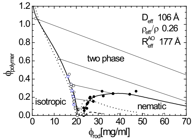
FIG. 5: Phase diagram for a mixture of fd virus and Dextran (MW 500,000, R_g = 176 \text{ \AA} or R^{AO} = 199 \text{ \AA} ) at 100 mM ionic strength. The measured points indicate the rod and polymer concentrations of the coexisting isotropic and nematic phases. The full line is a guide to the eye indicating the two phase region. Tie-lines are indicated by thin full lines. The SPTA and SVTA predictions are indicated by the dotted lines and dashed lines respectively. The polymer concentration is defined as follows \phi_{\text{polymer}} = \rho \frac{4\pi R_g^3}{3} .
