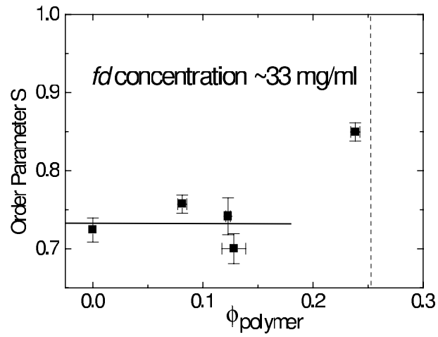
FIG. 8: Order parameter of the nematic phase at 33 mg/ml as a function of increasing polymer concentration for the fd and Dextran (M.W. 500 000) mixture at 100 mM ionic strength. The horizontal line drawn is a guide to the eye showing the independence of the nematic order parameter with polymer concentration. The vertical line indicates the location of the nematic-isotropic transition.
