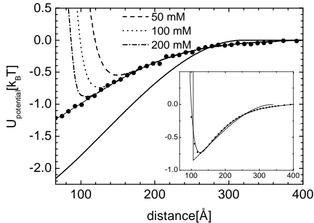
FIG. 3: Total interaction potential between two viruses ( D = 66 \text{ \AA} ) oriented at 90^\circ with respect to each other and immersed in a suspension of polymers of concentration \rho = 3/(4\pi R_g^3) and radius R_g = 111 \text{ \AA} at three different ionic strengths. The interaction potential is a sum of electrostatic repulsion and depletion interaction. For fd the electrostatic repulsive interaction is calculated as in [11, 32] with a net linear charge of 1 e^-/\text{\AA} . Filled circles indicate the depletion potential obtained from Monte Carlo simulation of polymers without excluded volume interactions. Since the polymer diameter is larger than the rod diameter, the polymer and rod-like viruses can easily interpenetrate. This results in an effective depletion attraction which is smaller than what is predicted by the AO model (indicated by the full line). The phase diagram corresponding to these interaction potentials are shown in Fig. 6. Inset : In theoretical calculations we approximate the intermolecular potential between rods with an effective hard core diameter D_{\text{eff}} [11] and attractive potential. The attractive part of the potential is modeled by AO penetrable spheres whose effective radius and concentration best fits the potential obtained through computer simulation. This effective intermolecular potential is compared to the potential obtained through the computer simulation in the inset. In the inset \rho_{\text{eff}}/\rho = 0.39 and R_{\text{eff}}^{\text{AO}} = 0.99 .
