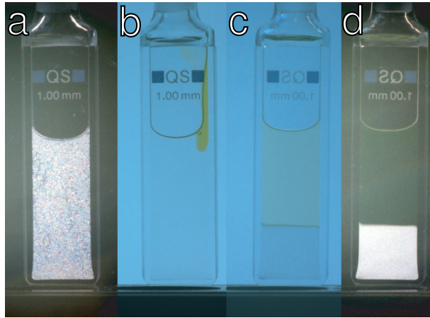
FIG. 1: a) A nematic liquid crystal of fd virus between crossed polarizers showing birefringent domains. b) A highly concentrated solution of Dextran labelled with yellow fluorescein is added to the transparent fd nematic liquid crystal. c) After a sample is vigorously shaken it phase separates into coexisting nematic and isotropic phases d) Image of the isotropic-nematic coexistence taken under crossed polarizers showing dense birefringent nematic phase on the bottom and polymer rich isotropic phase on the top.
