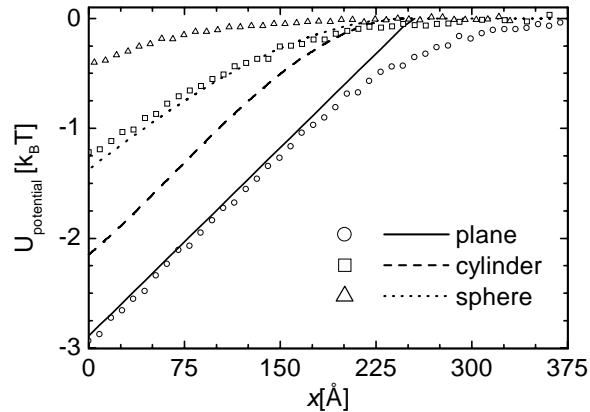
FIG. 2: Depletion potential between two walls, two perpendicular cylinders and two spheres obtained from computer simulation are shown by open spheres, squares and triangles respectively. In the two wall simulation the wall size was 313 \text{ \AA} long and no end effects were taken into account. The diameter of the spheres and cylinders is 66 \text{ \AA} while R_g of the polymer is 111 \text{ \AA} . The lines indicate depletion potentials as predicted by the penetrable sphere (AO) model. The separation x is the closest distance between two surfaces. The number concentration of the polymer \rho is equal to the overlap concentration \rho = 3/(4\pi R_g^3) , while the radius of the penetrable spheres is R^{\text{AO}} = 2R_g/\sqrt{\pi} = 125 \text{ \AA} . The AO theory overestimates the potential between spheres and polymers because polymer can deform around colloidal particles.
